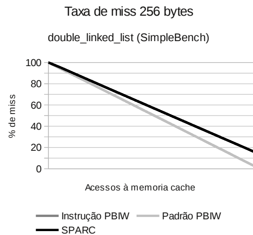
(A.6) double_linked_list
