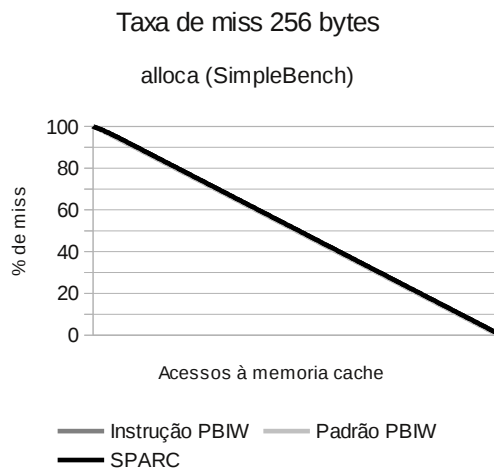
(A.1) alloca
