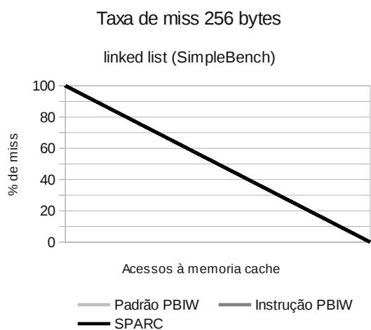
(A.9) list_list
