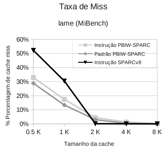
(A.21) lame
