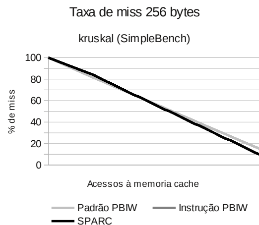
(A.8) kruskal
