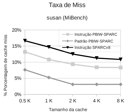
(A.27) susan
