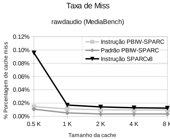
(A.37) rawaudio
