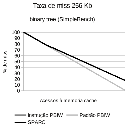
(A.3) binary_tree
