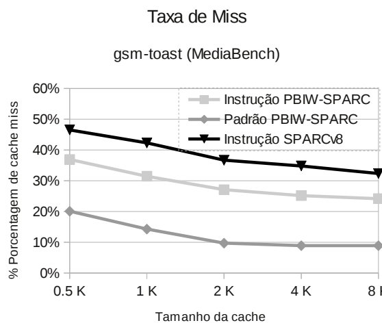
(A.39) toast
