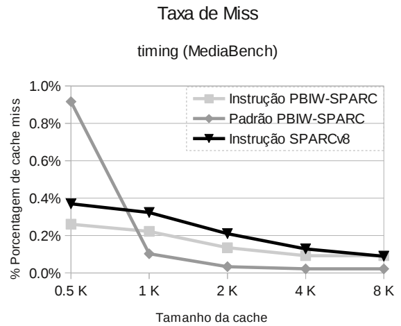
(A.38) timing
