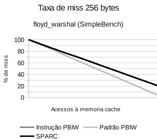
(A.7) floyd_warshall
