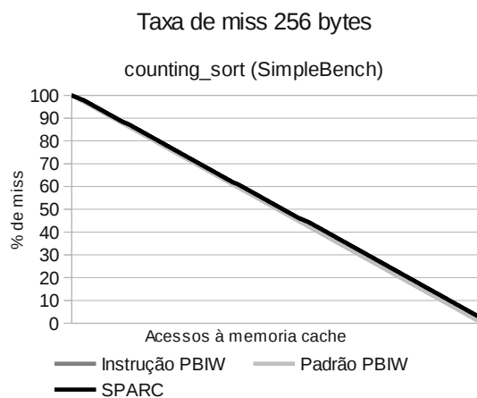
(A.5) counting_sorte
