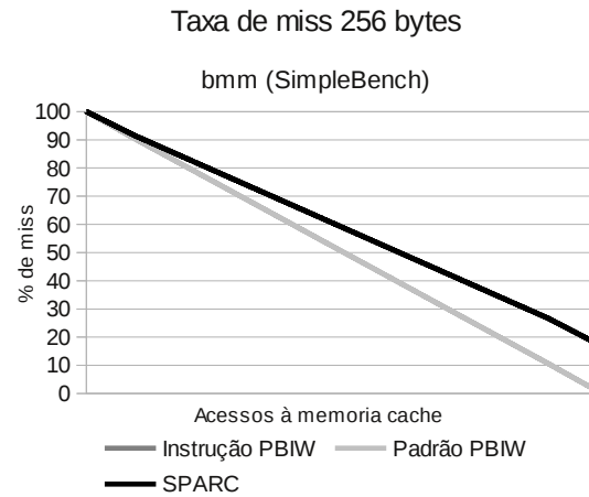
(A.4) bmm
