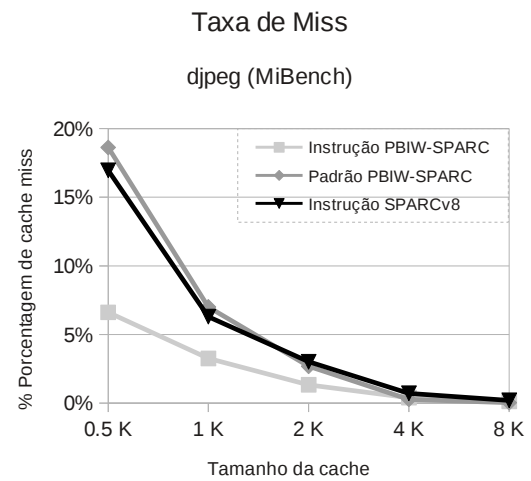
(A.19) djpeg
