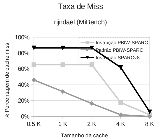
(A.25) rijndael
