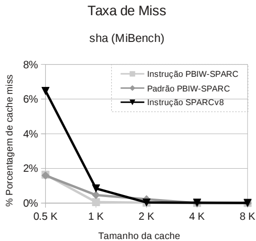
(A.26) sha
