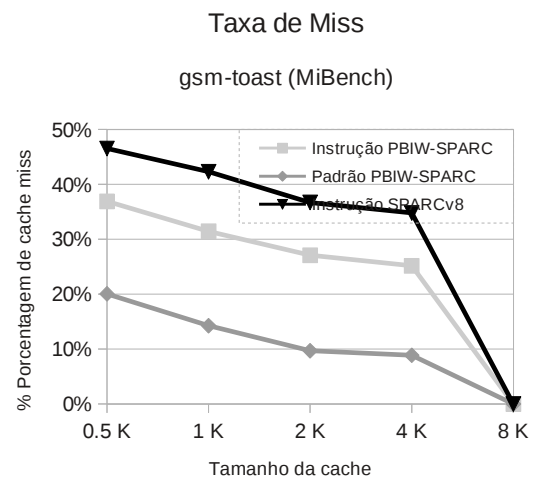
(A.29) toast
