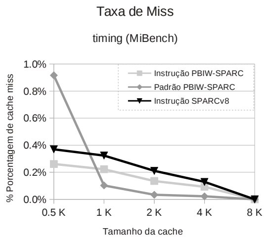
(A.28) timing
