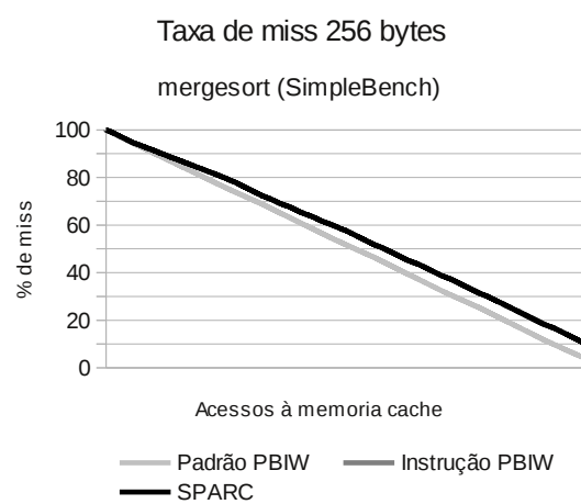
(A.10) mergesort
