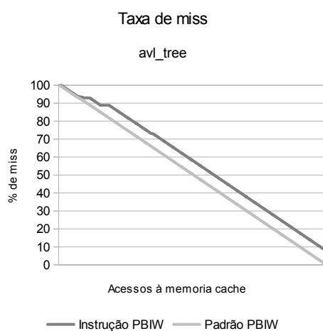
(a) avl_tree
