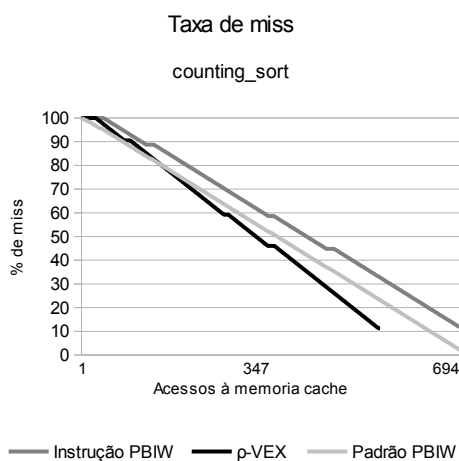
(c) counting_sort
