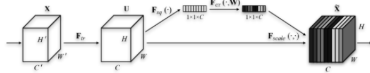
Figura 3.6: Bloco Squeeze-and-Excitation da SE-ResNeXt.
