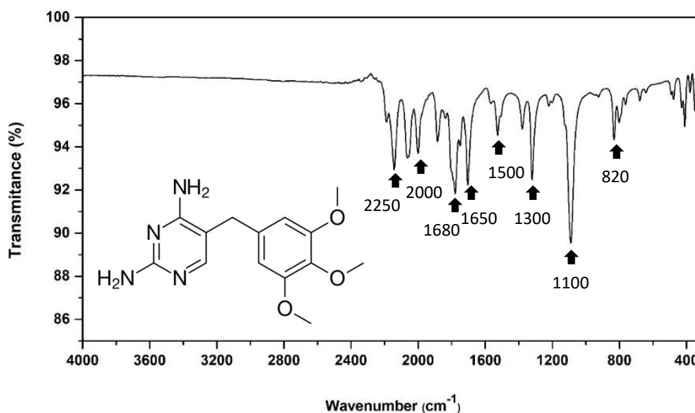
Figure 10. Absorption spectrum in the infrared region of the raw material trimethoprim obtained in the range of 4000-500 \text{cm}^{-1} with the Attenuated Total Reflection (ATR) technique and the iD3 ® accessory with Germanium crystal.
