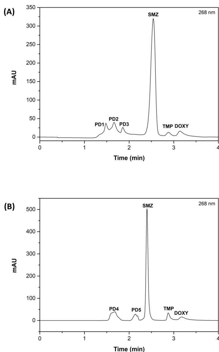
Figure 25. Chromatograms of the combination of sulfamethazine (SMZ), trimethoprim (TMP) and doxycycline (DOXY); (A) basic hydrolysis (0.01 M NaOH, 4 h), (B) acid hydrolysis (0.1 M HCl, 8 h), (C) oxidative hydrolysis (0.03% H 2 O 2 , 30 min), (D) neutral hydrolysis (H 2 O, 30 min); (E) Photolysis (UV/VIS light, 16 h). Chromatographic conditions: Macherey-Nagel (MN) C8 analytical column (4 mm x 125 mm, 5 \mu m), flow rate of 0.5 mL min -1 and mobile phase composed of acetonitrile:water (45:55 v/v) with pH adjusted to 3.0.
