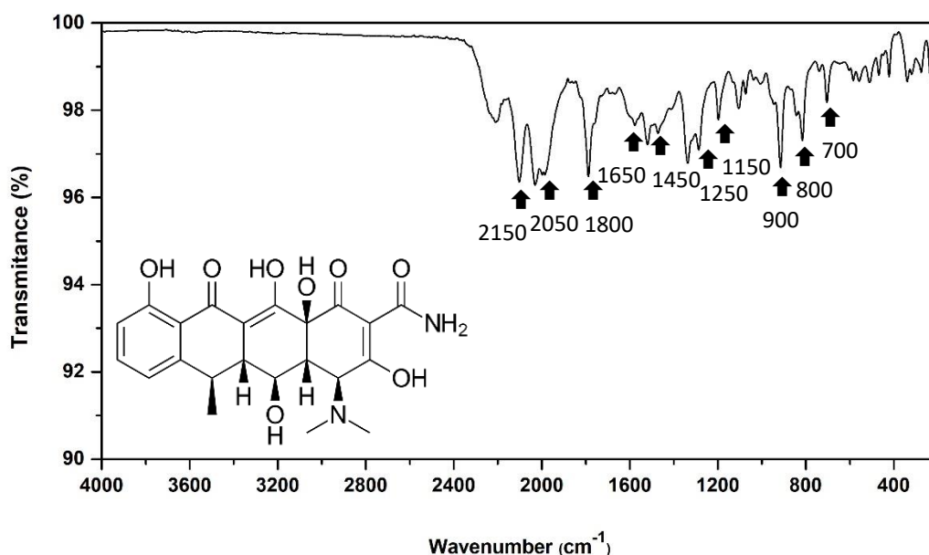
Figure 12. Absorption spectrum in the infrared region of the raw material doxycycline obtained in the range of 4000\text{--}500\text{ cm}^{-1} with the Attenuated Total Reflection (ATR) technique and the iD3 ® accessory with Germanium crystal.
