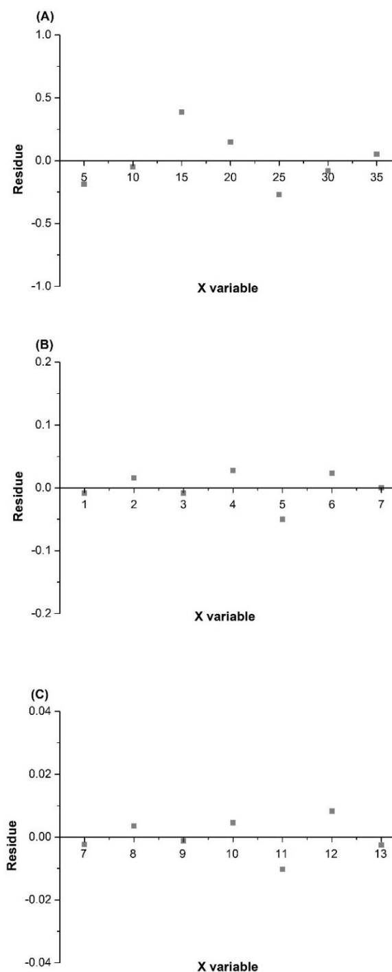
Figure 22. Analysis of residues obtained from the calibration curves of (A) SMZ (sulfamethazine), (B) TMP (trimethoprim) and (C) DOXY (doxyxycine).
