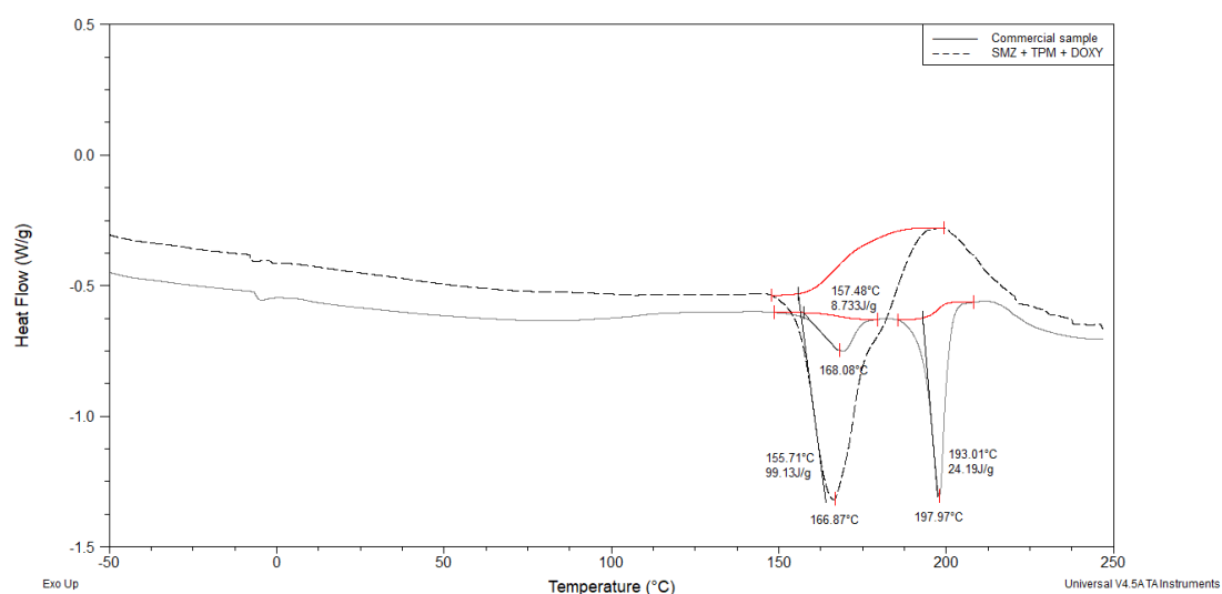
Figure 34. DSC (flow rate of 60.0 \text{ mL min}^{-1} and temperature range from -50 to 250^\circ\text{C} ) curves of the commercial sample and ternary mixture of sulfamethazine (SMZ), trimethoprim (TMP) and doxycycline (DOXY) ( 1:1:1 \text{ m/m/m} ) obtained in a nitrogen atmosphere under a heating rate of 10^\circ\text{C min}^{-1} .
