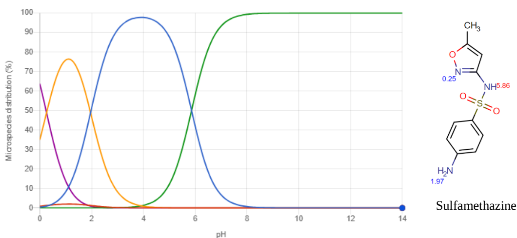
Figure 16. Distribution of sulfamethazine microspecies (%) as a function of pH.
