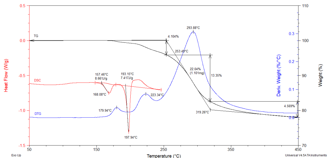
Figure 32. TG/DTG (flow rate of 40.0 mL min -1 up to 450°C) and DSC (flow rate of 60.0 mL min -1 and temperature range from -50 to 250°C) curves of the commercial sample obtained in a nitrogen atmosphere under a heating rate of 10°C min -1 .
