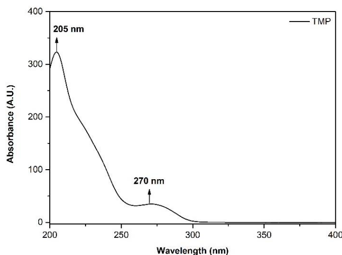
Figure 9. Absorption spectrum in the UV/Vis region of the raw material trimethoprim (TMP) using acetonitrile:water (45:55 v/v) as solvent.
