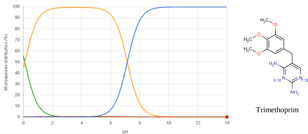
Figure 17. Distribution of trimethoprim microspecies (%) as a function of pH.
